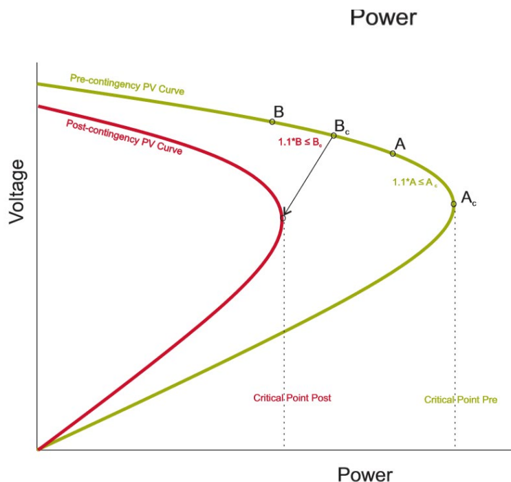
Figure 4-14-1: Typical PV Power-Voltage Curves
