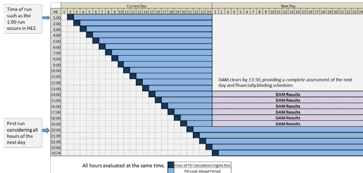
Figure 2-3: Future PD Calculation Engine Run Timing and Multi-Hour Look-Ahead Period
