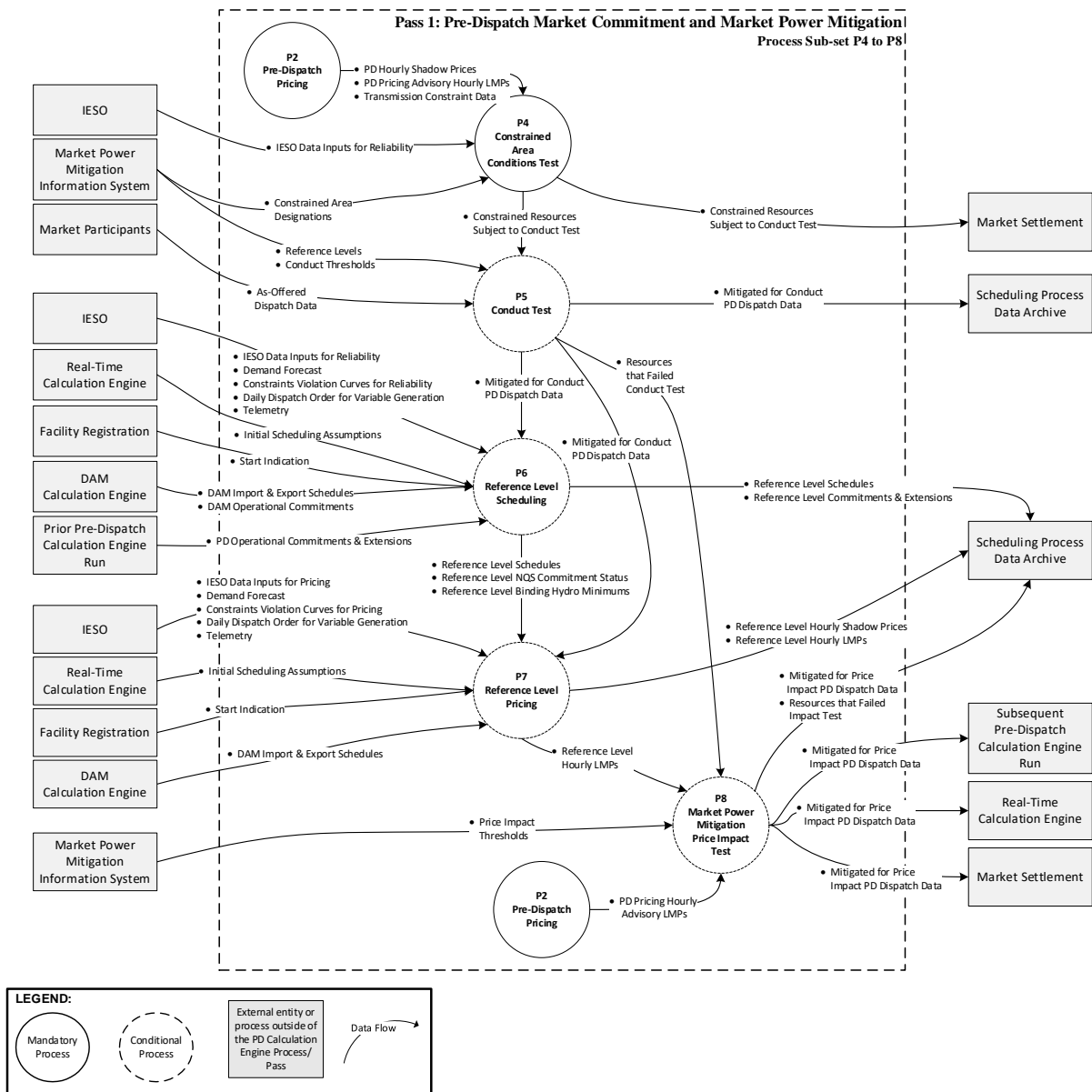
Figure 6-3: Level 1 Information Flow Diagram for Sub-Set of Pass 1 – P4 to P8
