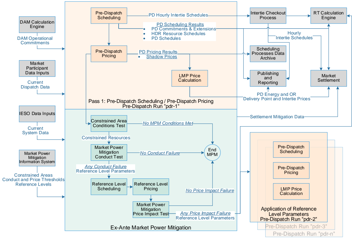
Figure 2-4: Future PD Calculation Engine Processes
