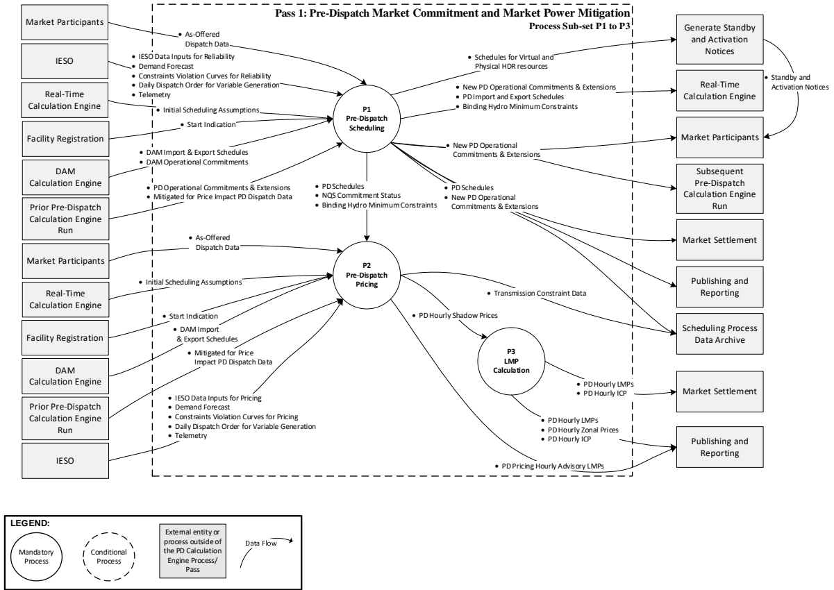
Figure 6-2: Level 1 Information Flow Diagram for Sub-Set of Pass 1 - P1 to P3
