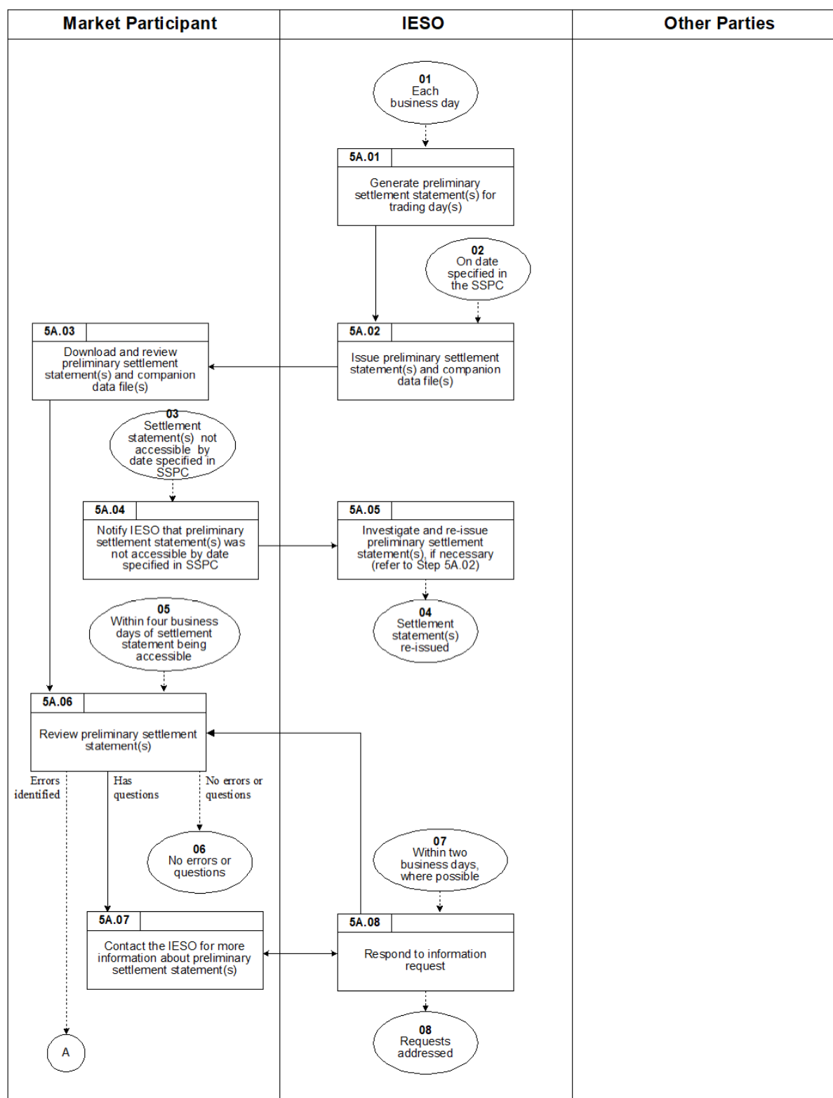
Figure 2–1: Work flow for Preliminary Settlement Statements
