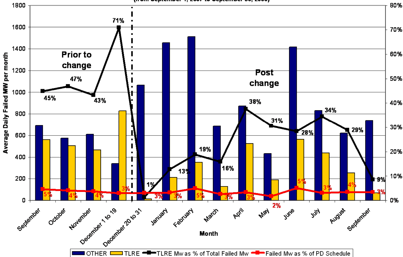
Failed MW between Ontario and New York (from September 1, 2007 to September 30, 2008)
