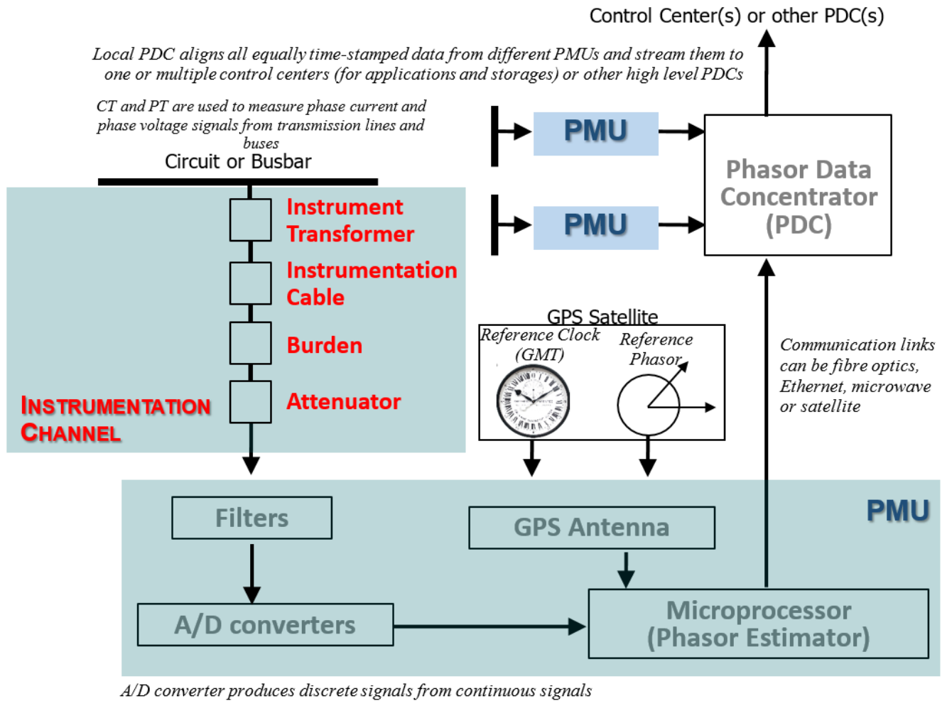
Figure 1 | Typical infrastructure required for providing synchrophasor data
