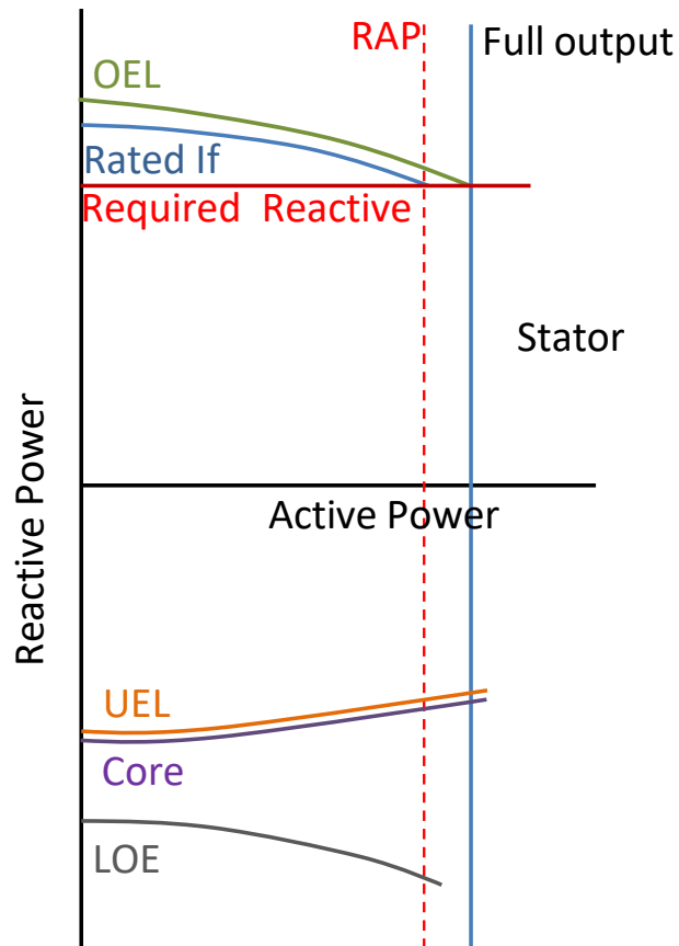
Figure 19 - Capability Curve
