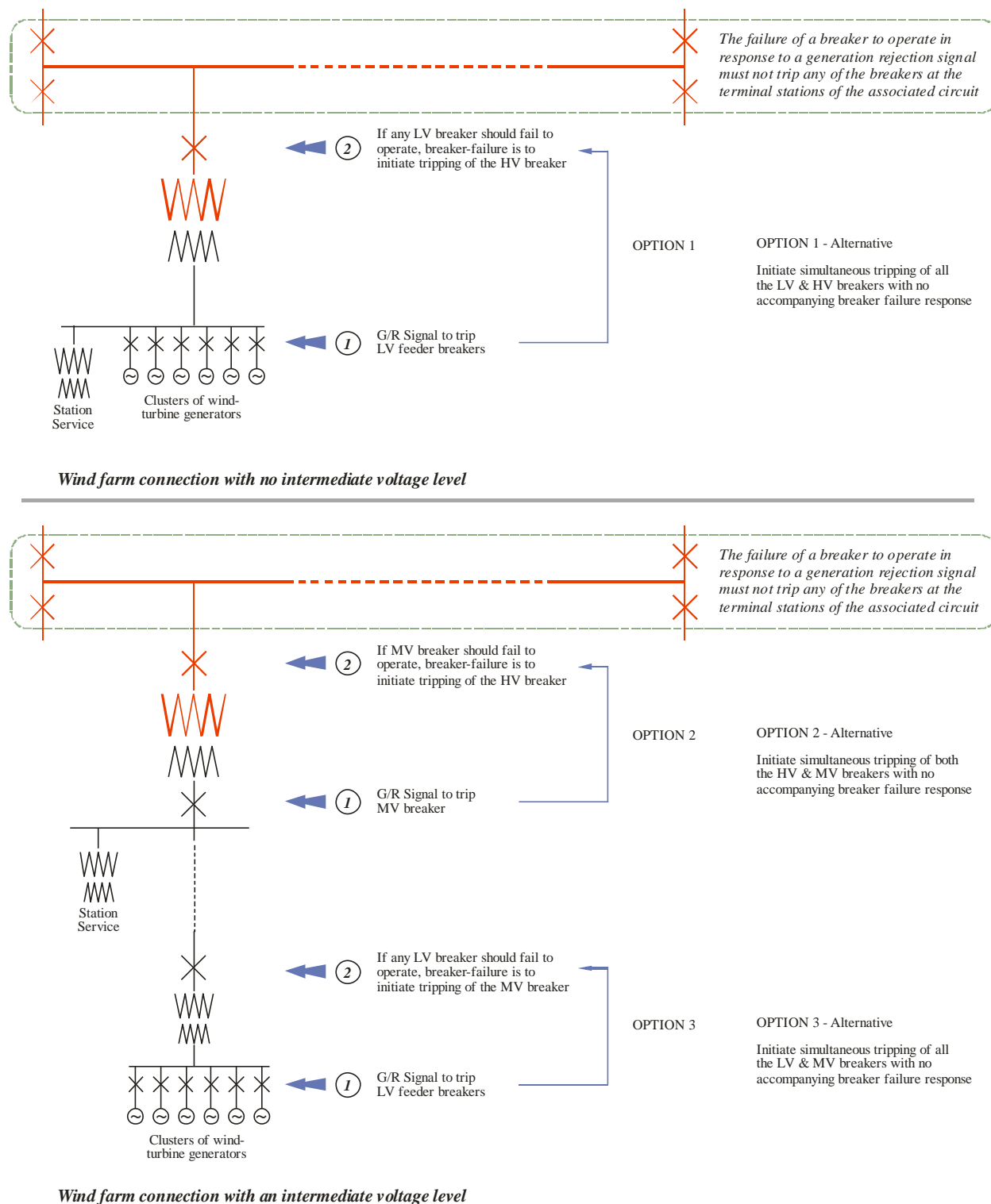
Typical Connection Arrangements for Wind Farms with suggested generation rejection responses
