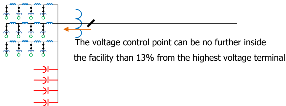
Figure 14 - Voltage Control Point
