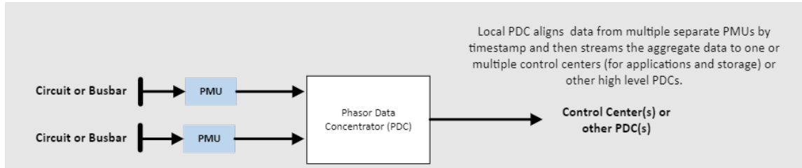
Figure 5-2: Typical infrastructure for multiple PMUs
