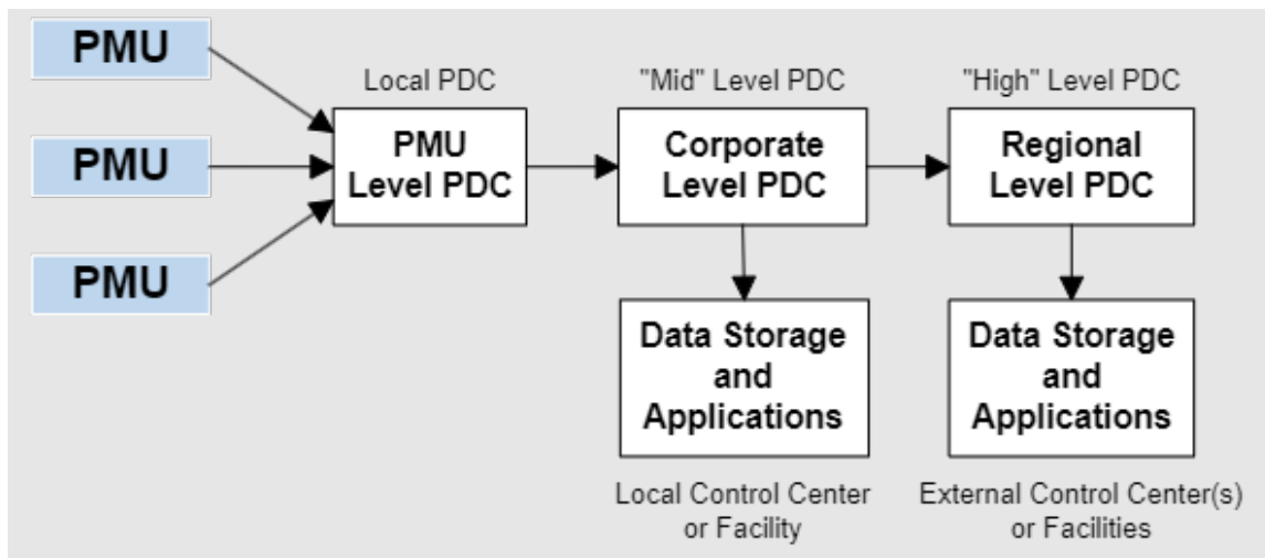
Figure 5-3: PMU and Phasor Data Concentrators
