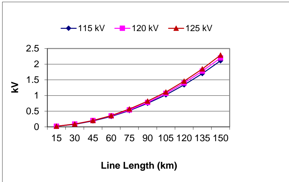
Figure 4: 115 kV LEO Voltages
