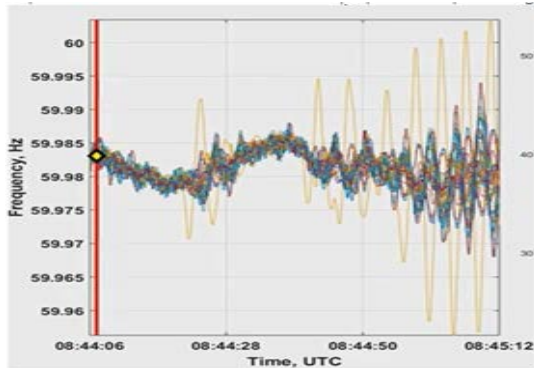
Frequency from Ontario SCADA
