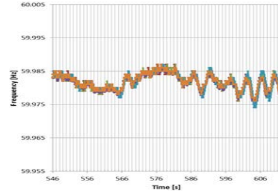
Frequency from Ontario DDR and DFR
