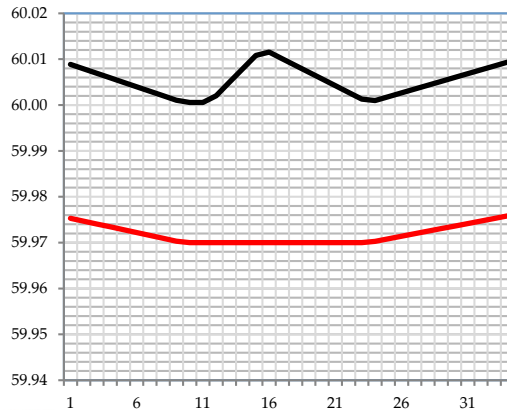
Frequency from Ontario SCADA
