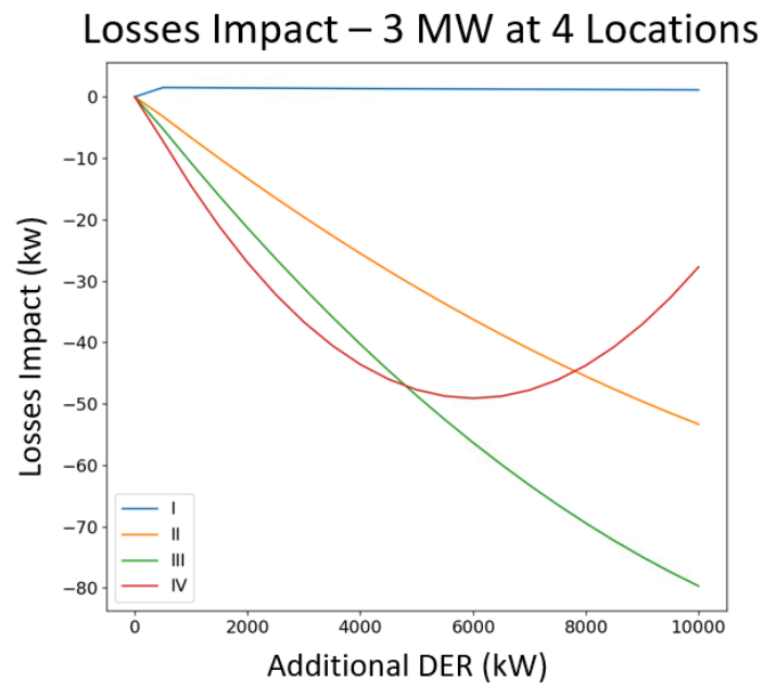
Figure 5-5. Range of Losses Impacts Across Feeder 1
