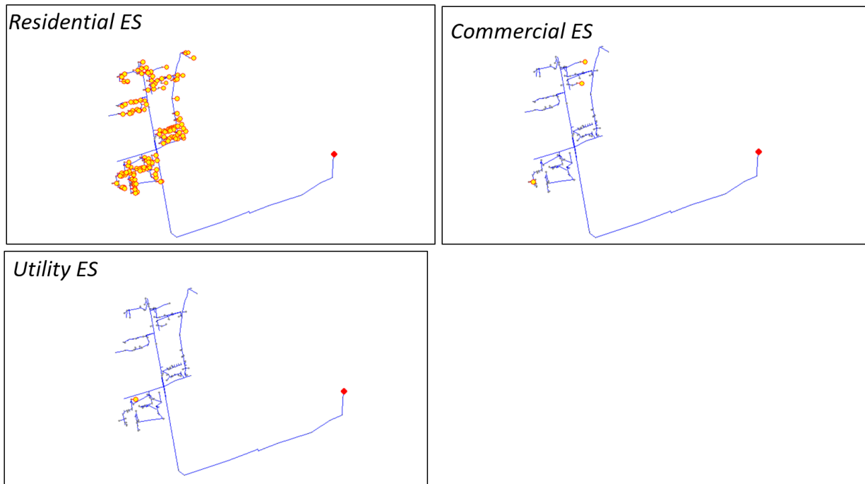
Figure 5-17. Energy Storage Allocations for Feeder 2 (DER scales: residential (top left), commercial (top right), utility (bottom))
