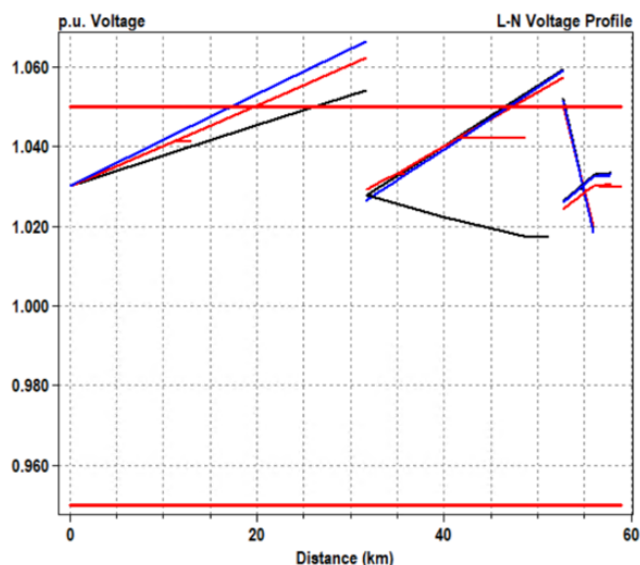
Figure 5-9. IEEE 34-bus Voltage Profile at Minimum Load with DER (Full Output)
