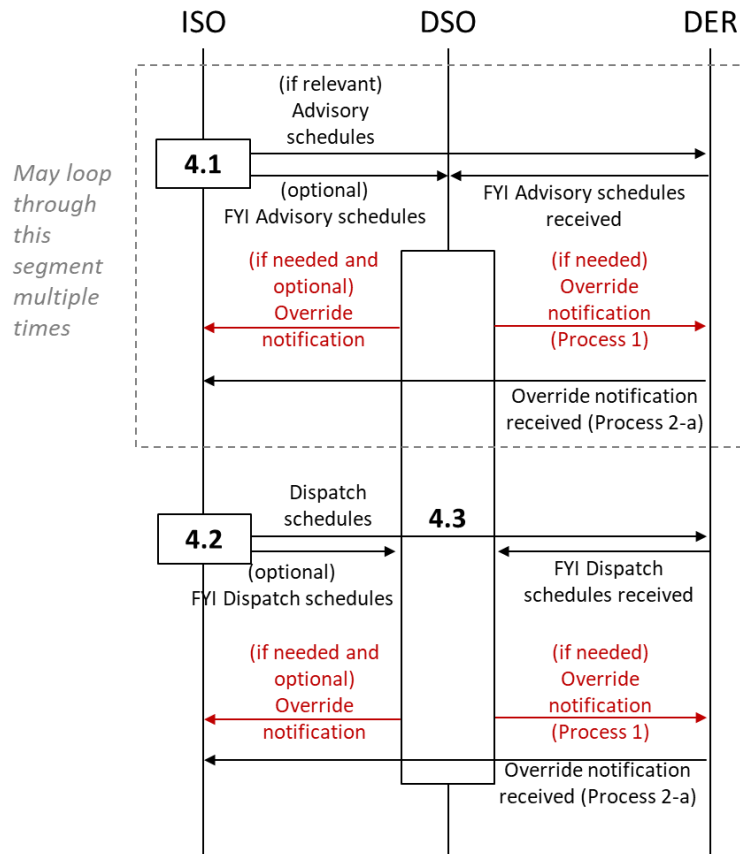
Figure 4-20. Sequence diagram, Stage 4 with Dual Participation model
