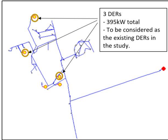
Figure 5-19. Feeder 3 Topography with Existing DER Locations Identified
