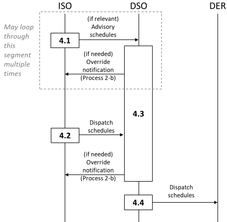
Figure 4-10. Sequence diagram, Stage 4 with Total DSO model.
