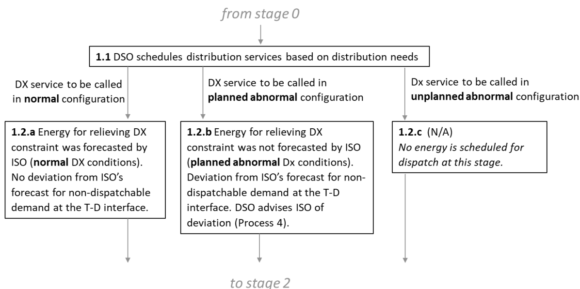
Figure 4-5. Functional diagram, Stage 1 with Total DSO model
