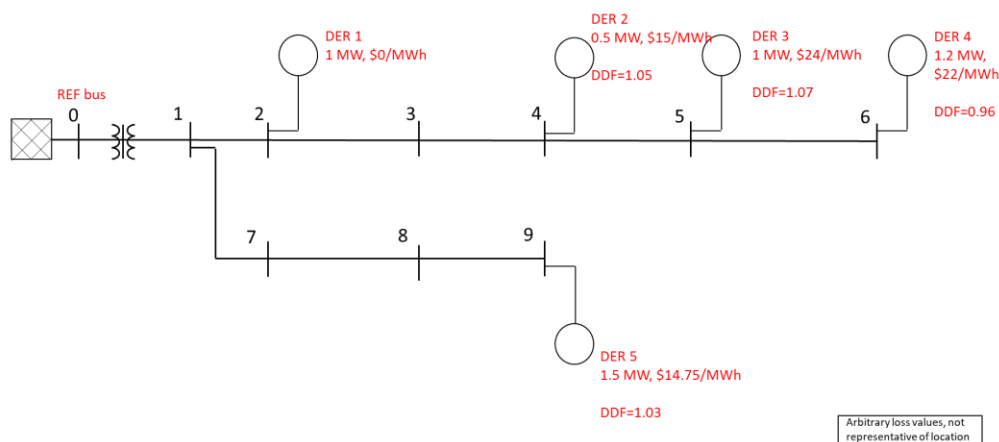
Figure 6-1. Nine bus test feeder with DER details
