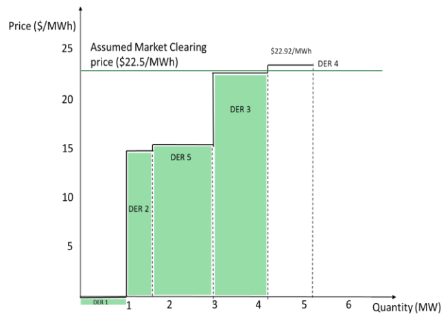
Figure 6-2. One single offer with multiple price-quantity pairs provided by DER/DERA or DSO
