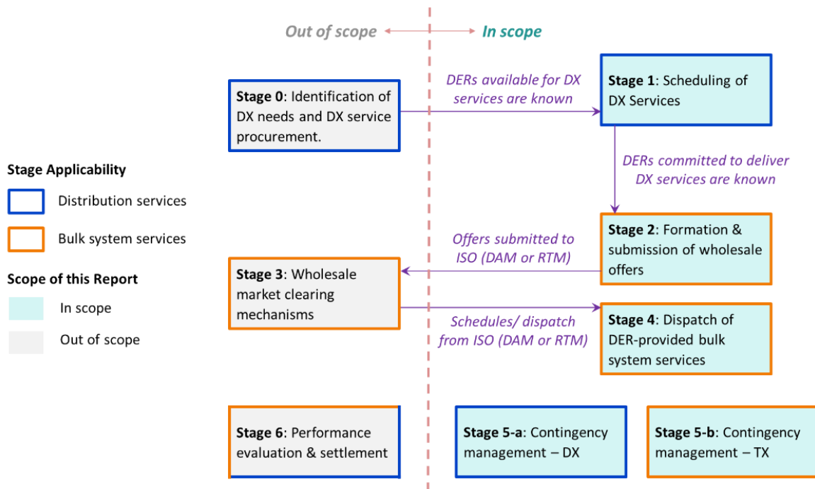
Figure 4-2. Coordination stages considered.
