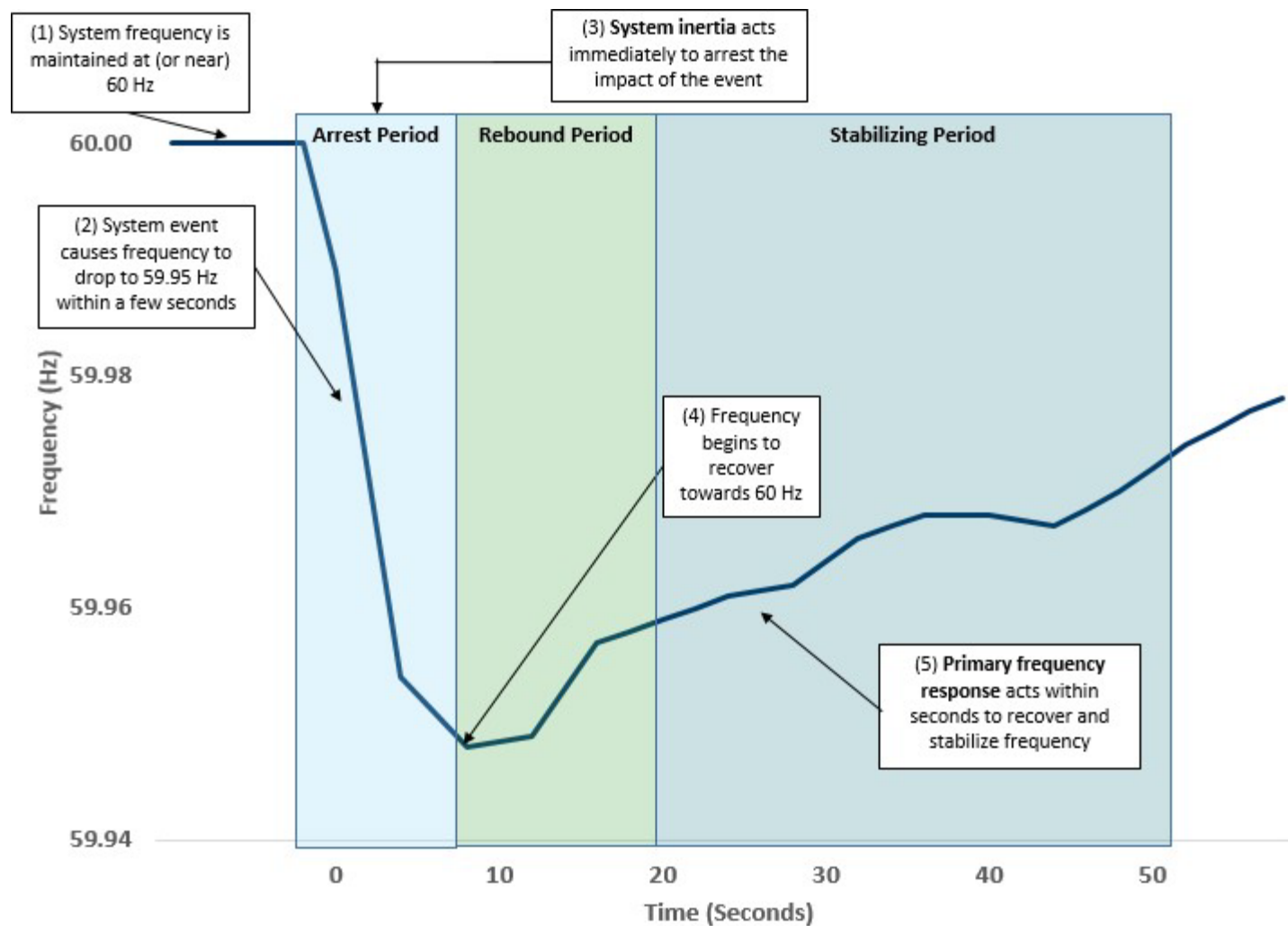
Figure 3 | Frequency Response
