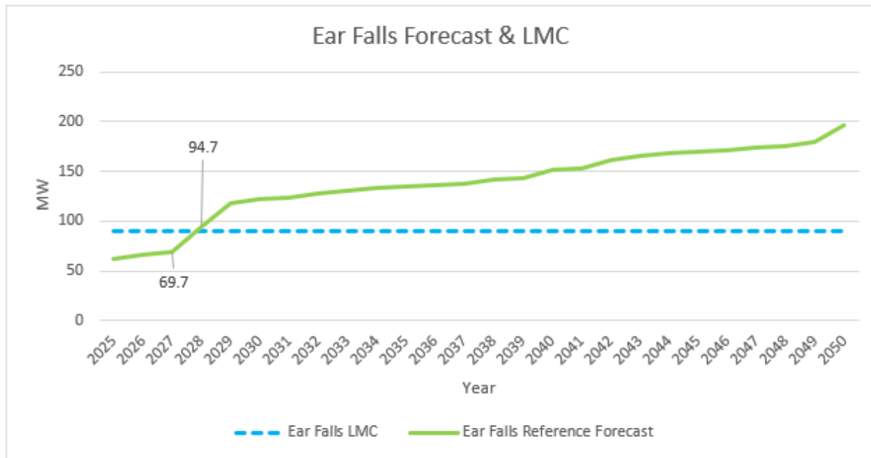
Figure 6.4 | Flow into Ear Falls Load Meeting Capability and Forecast Scenarios
