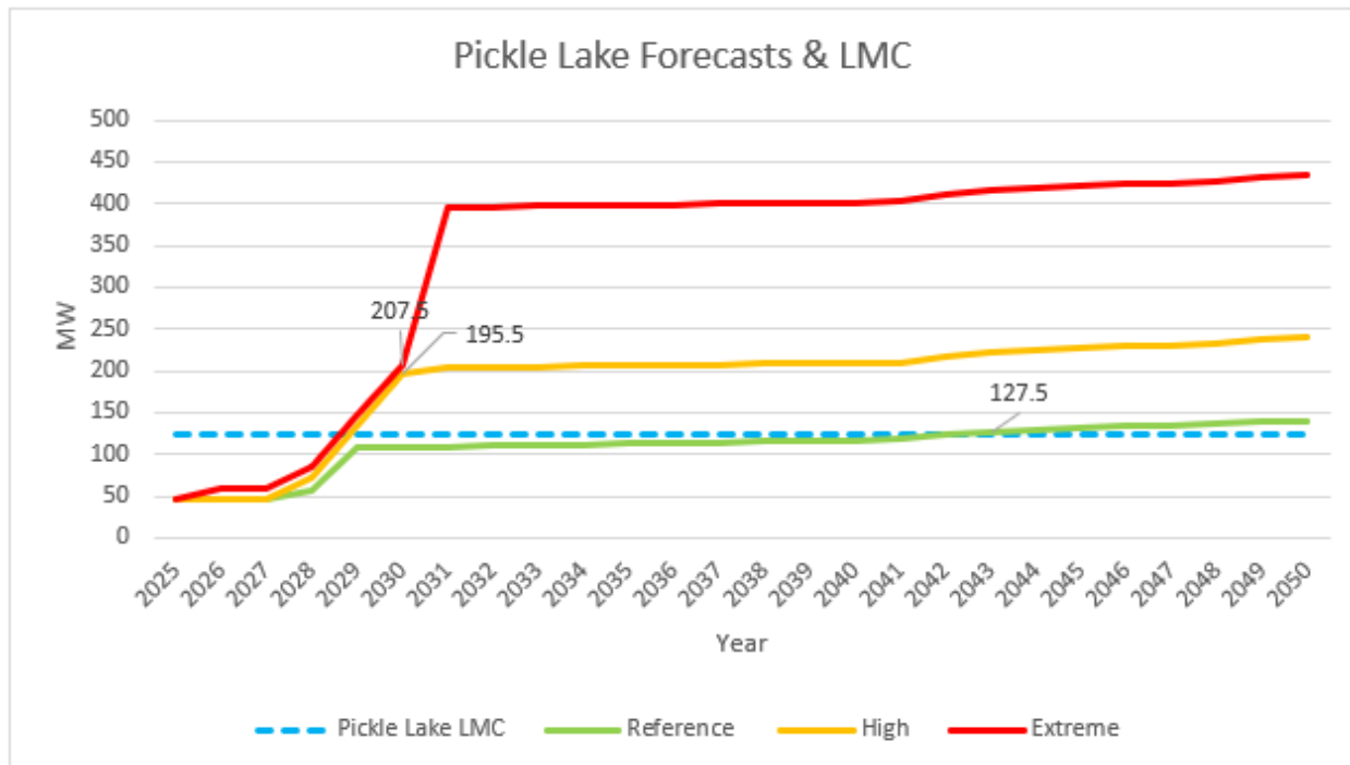
Figure 6.3 | Flow into Pickle Lake Load Meeting Capability and Forecast Scenarios
