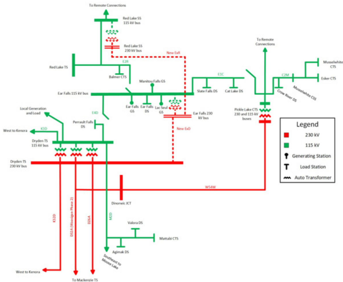
Figure 7.3 | Transmission Option 3
