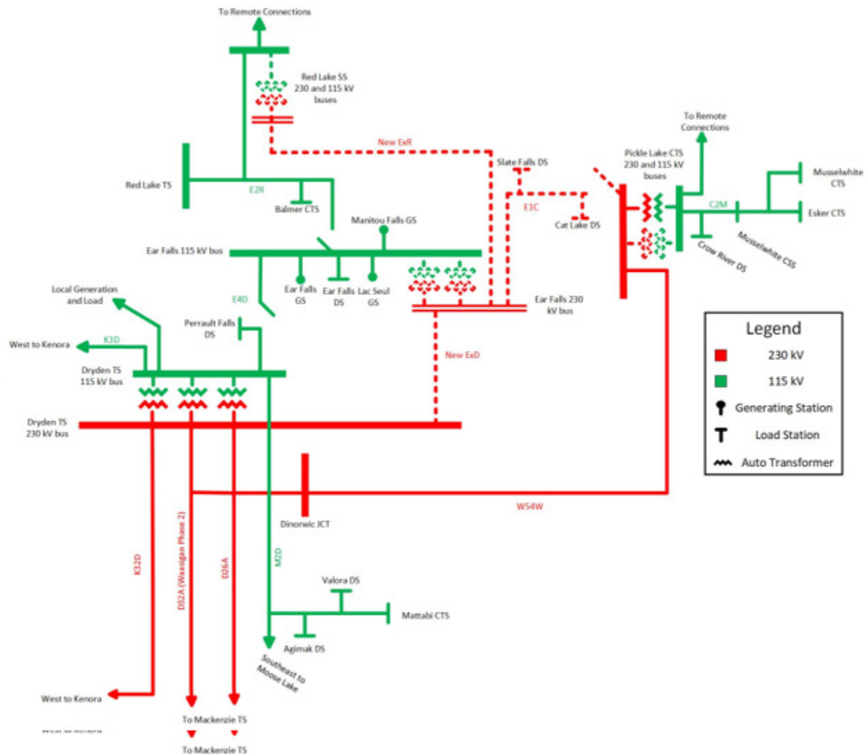
Figure 7.2 | Transmission Option 2
