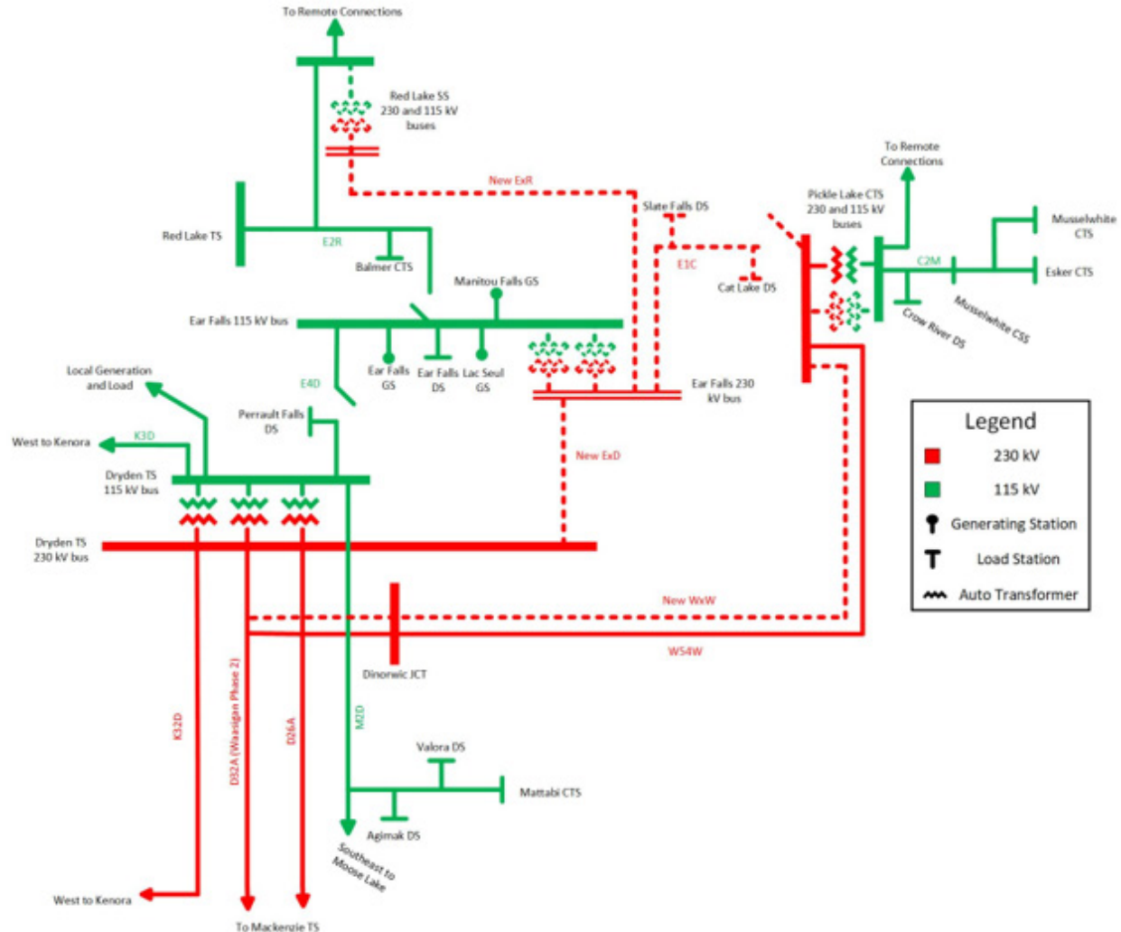
Figure 7.1 | Transmission Option 1
