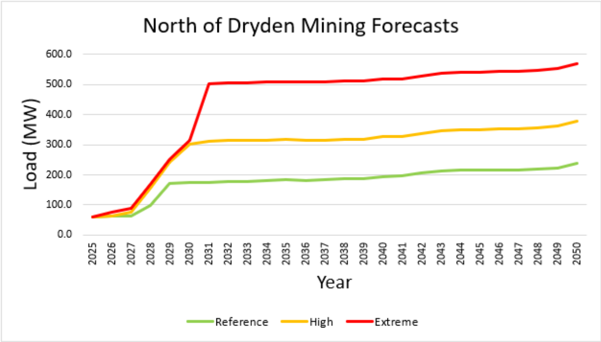
Figure 5.4 | Mining Demand Forecast
