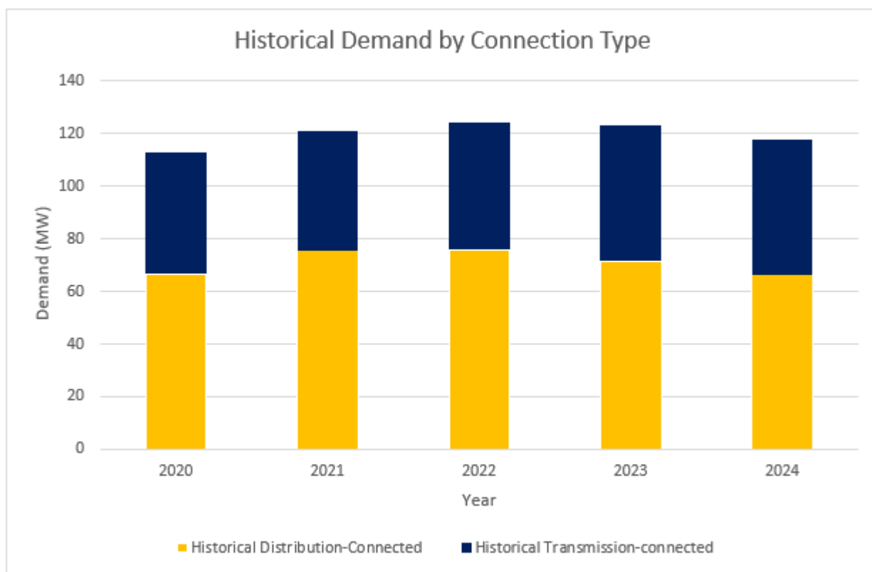
Figure 5.1 | 2020–2024 Historical Demand
