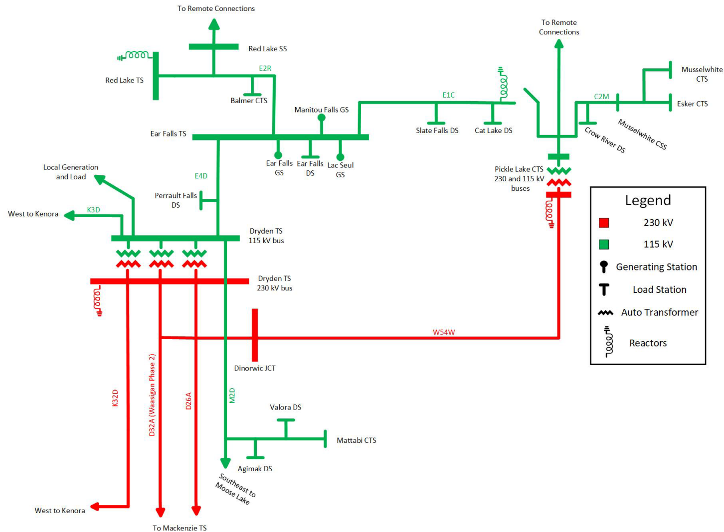
Figure 1.2 | Current Electricity Infrastructure in the North of Dryden Sub-Region
