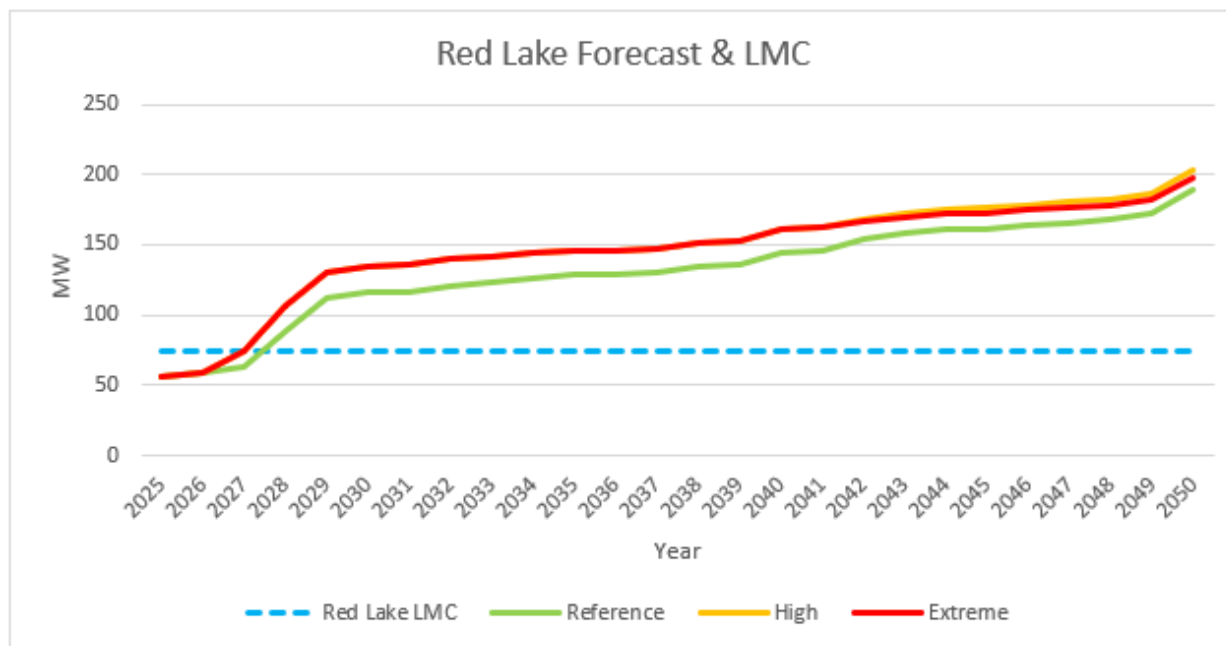
Figure 6.5 | Red Lake Load Meeting Capability and Forecast Scenarios
