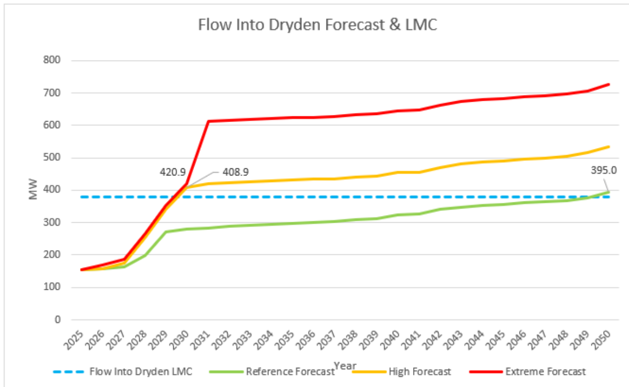
Figure 6.2 | Flow into Dryden Load Meeting Capability and Forecast Scenarios
