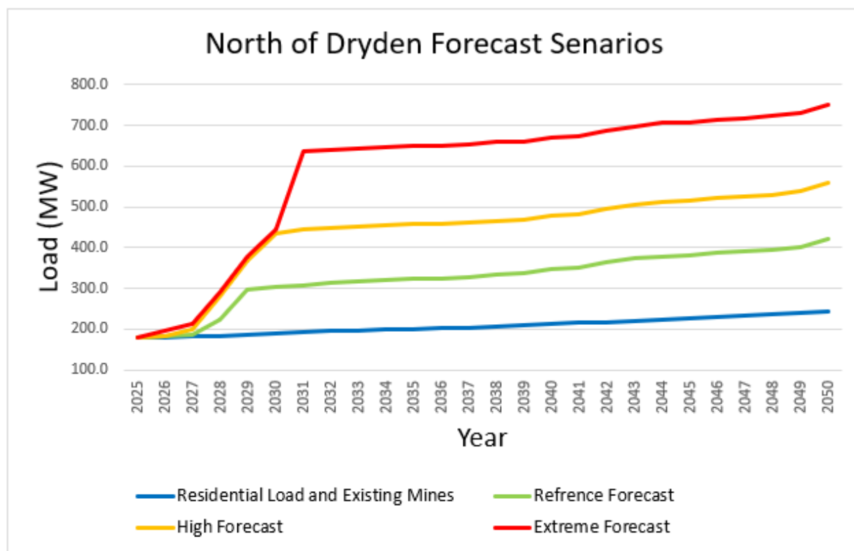
Figure 5.5 | Total North of Dryden Demand Forecast
