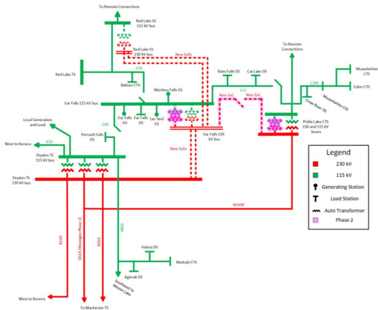
Figure 7.4 | Transmission Option 3 Double Circuit
