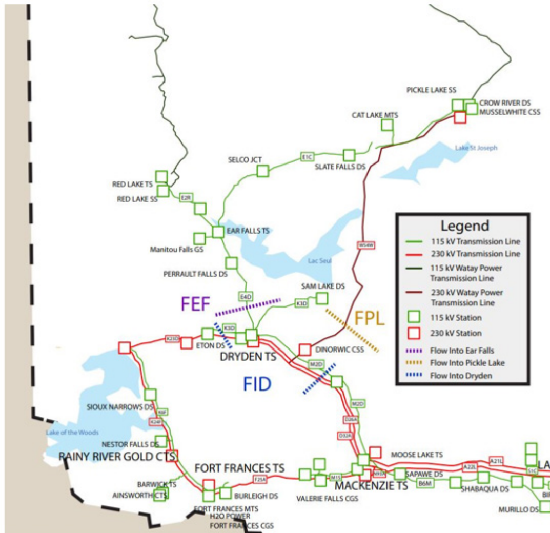
Figure 6.1 | North of Dryden Interfaces
