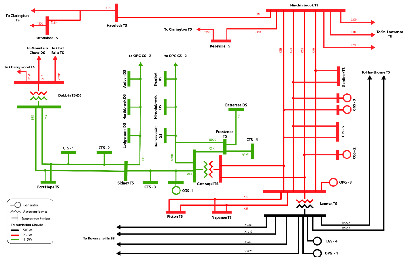
Figure 3 | Single line diagram of Peterborough to Kingston Region
