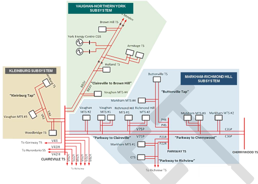
Figure B-2: Single Line Diagram of GTA North (York Region)
