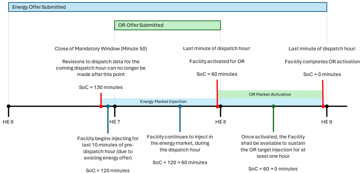
Figure 5 | Generator Resource Available Energy
