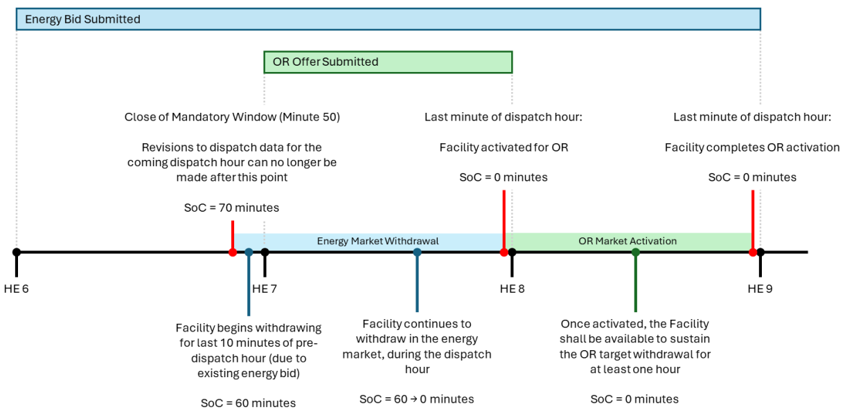
Figure 6 | Load Resource Available Energy
