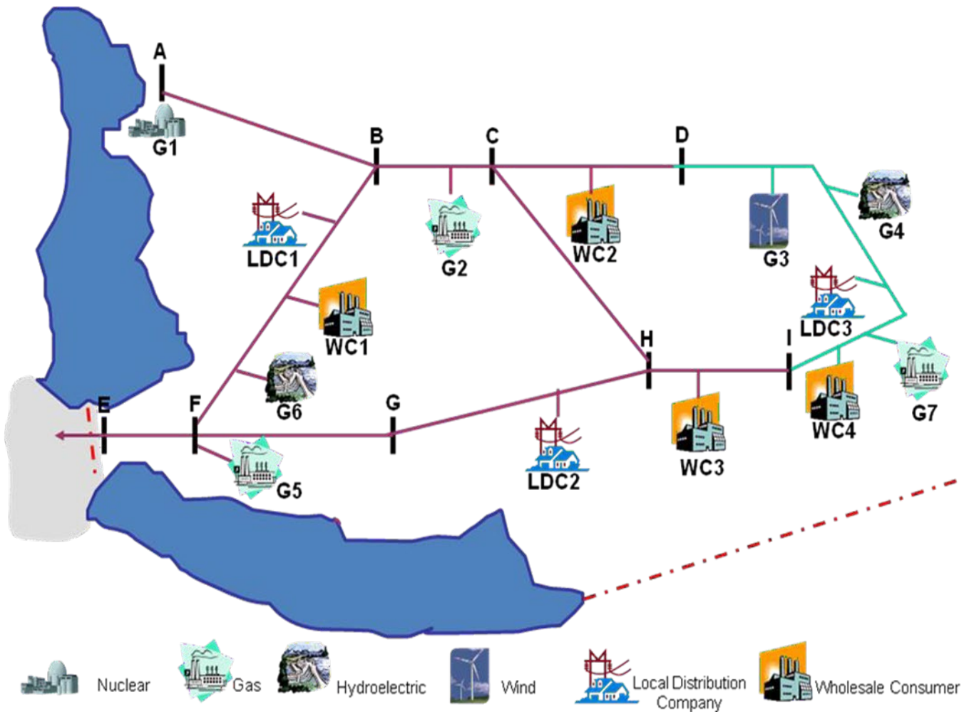
6.1 Figure 1: Generic Power System
