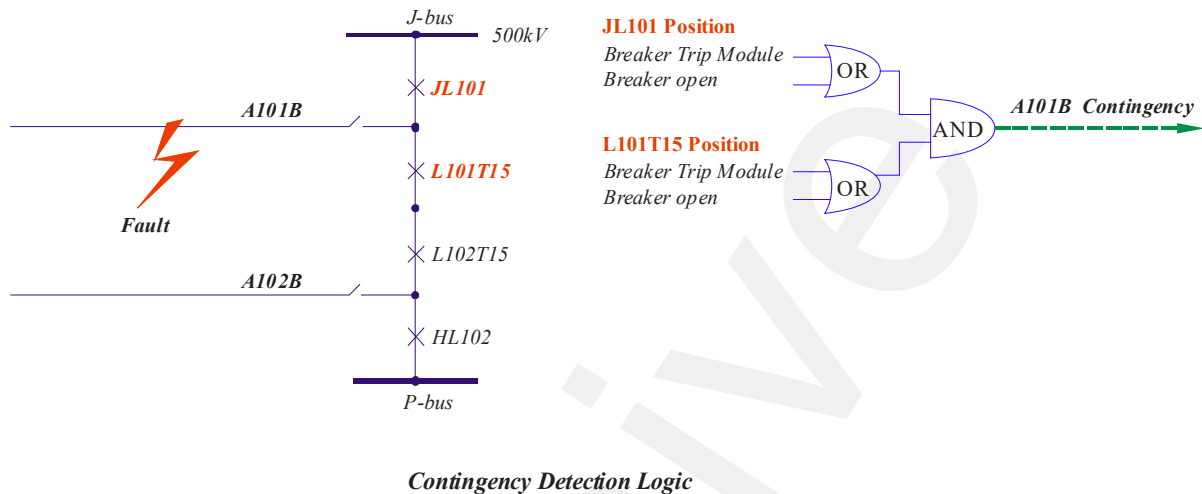
Figure 21 - Contingency Detection Logic
