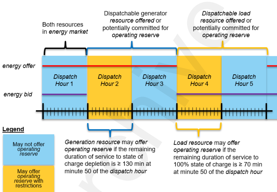
Figure A-1: Electricity Storage Dispatch Data Example
