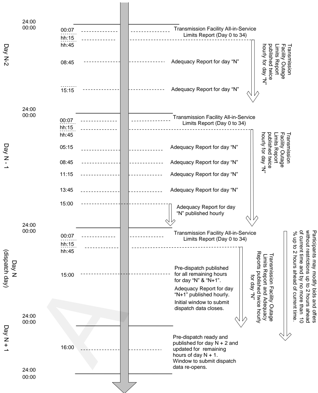
Figure E-1: Adequacy Report, Transmission Limits Report, Pre-dispatch and Dispatch Process Coordination Timing Chart
