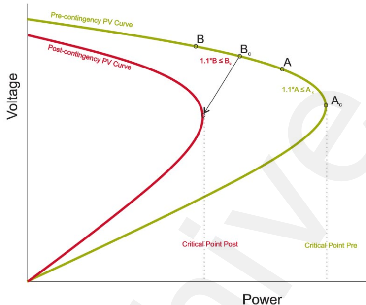
Figure 4-1: Typical Power-Voltage Curves
