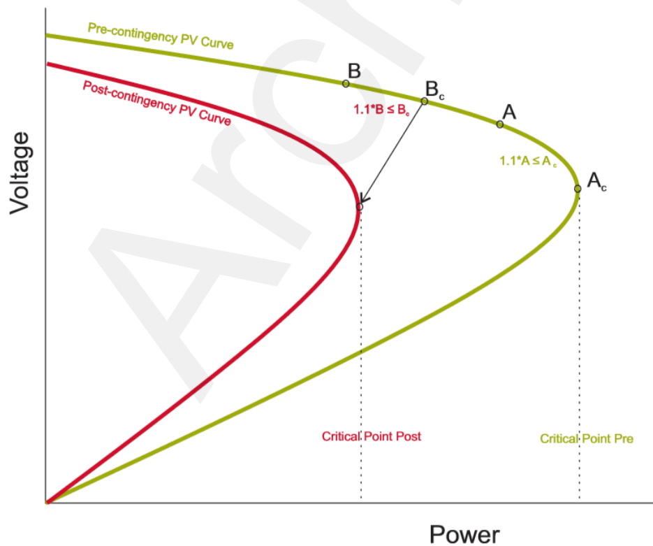
Figure 4-1: Typical PV Curves
