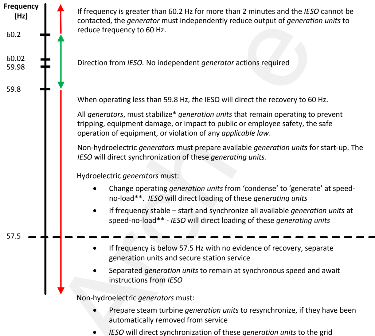
Figure 5: Generator Actions During Abnormal Frequency
