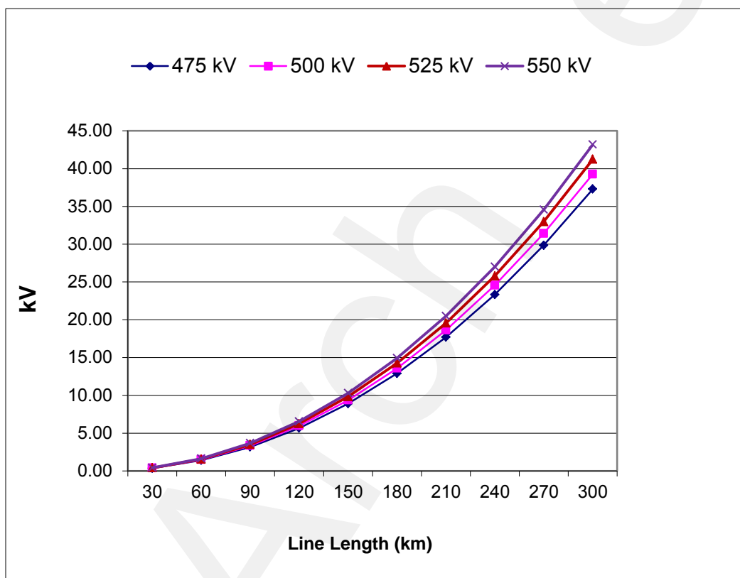
Figure 2: 500 kV LEO Voltages
